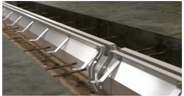
SILICON SEALANT APPLIED AND BOLTED BETWEEN ONE DRAIN FLANGES
