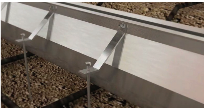
THREADED ROD CONNECTION BETWEEN LEVELING BRACKET AND THE CONCRETE BASE
