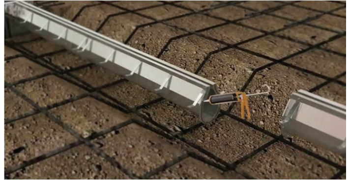
SILICON SEALANT APPLIED IN THE FLANGES BETWEEN DRAIN CONNECTIONS
