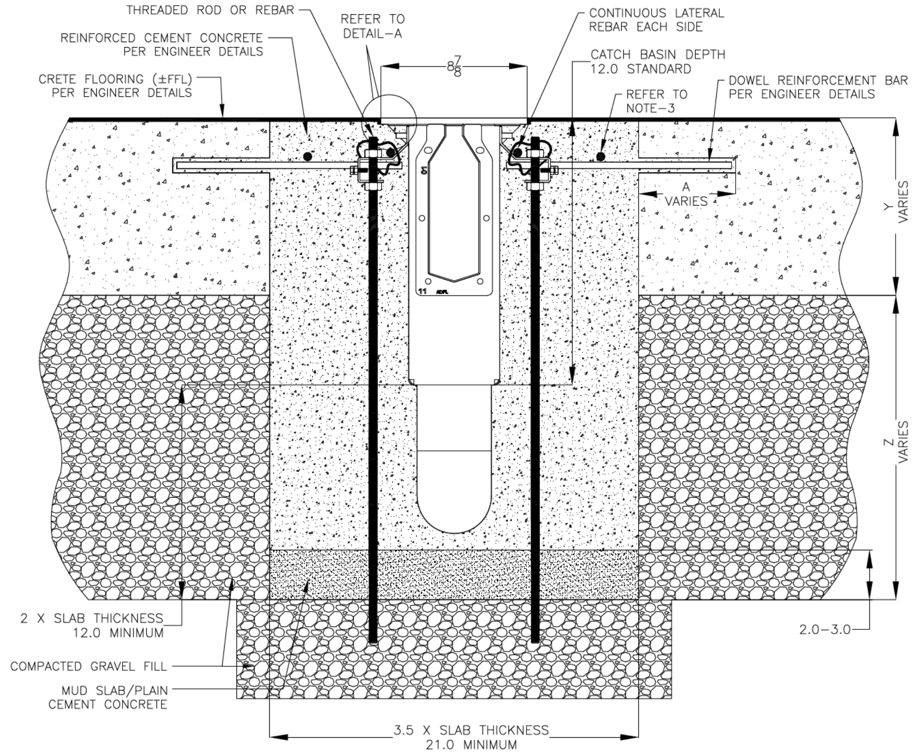
6X12X12 CATCH BASIN INSTALLATION DETAILS
