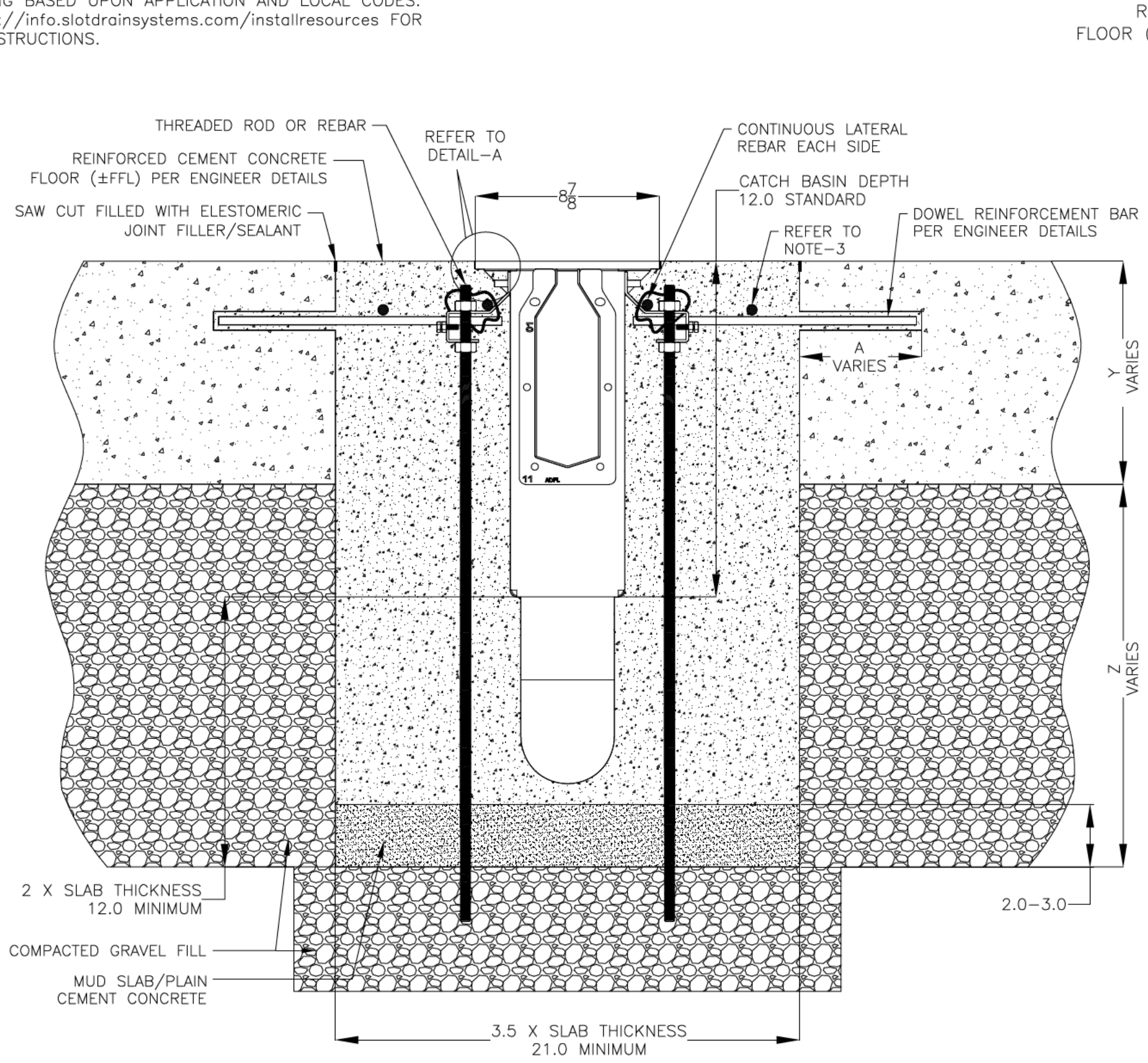
6X12X12 CATCH BASIN INSTALLATION DETAILS
