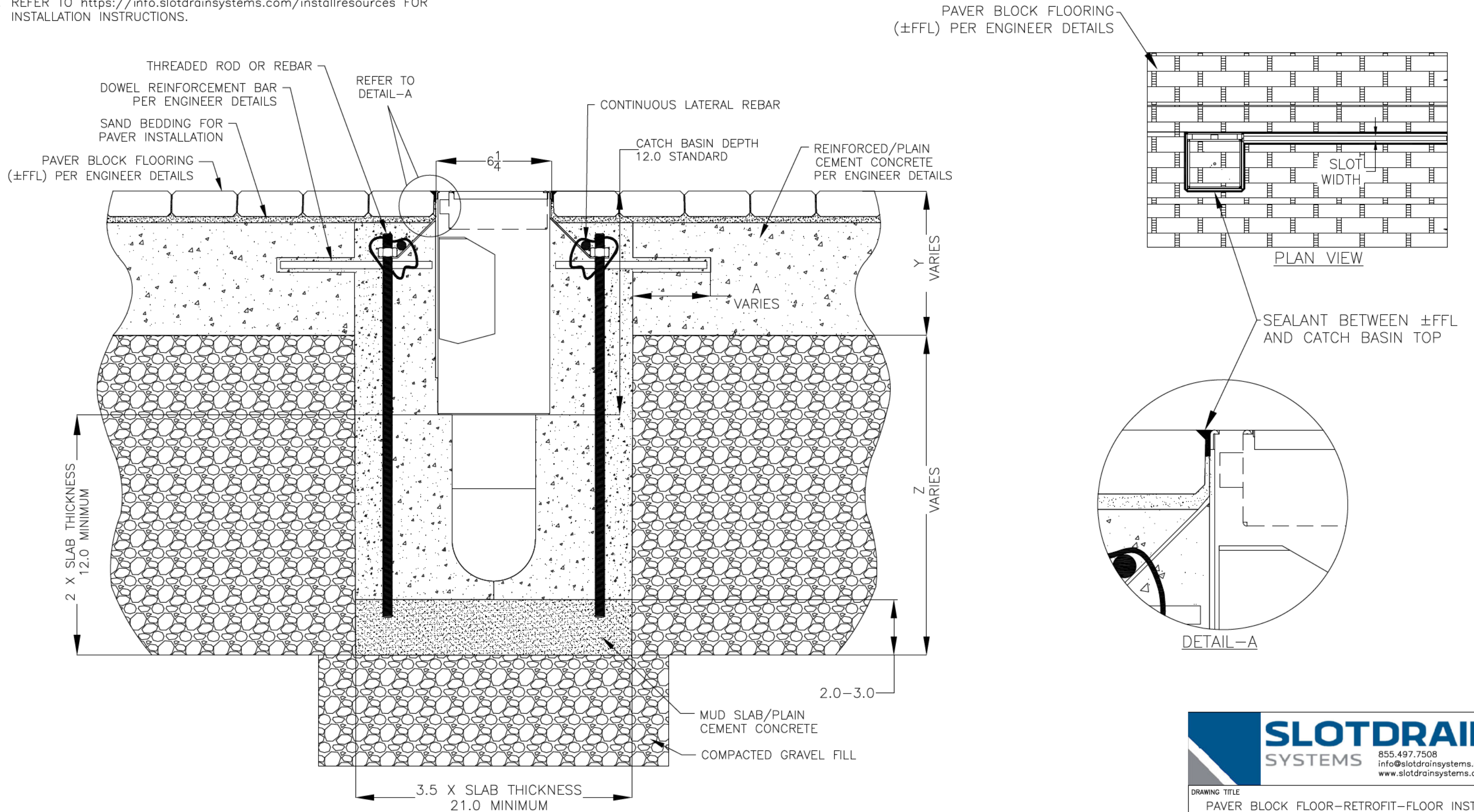
6X6X12 NON FG 4000 CATCH BASIN INSTALLATION DETAILS
