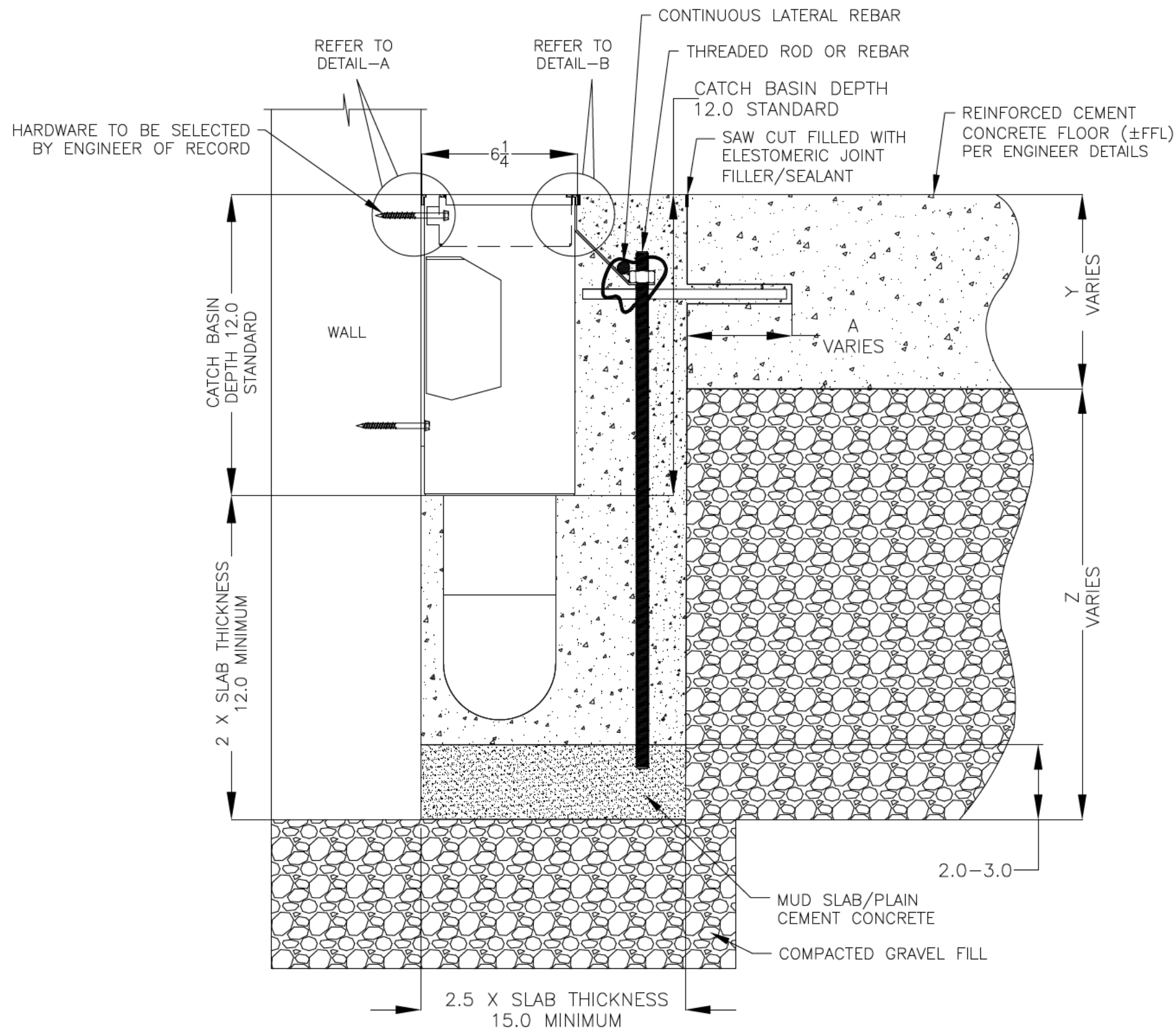
6X6X12 NON FG 4000 CATCH BASIN INSTALLATION DETAILS
