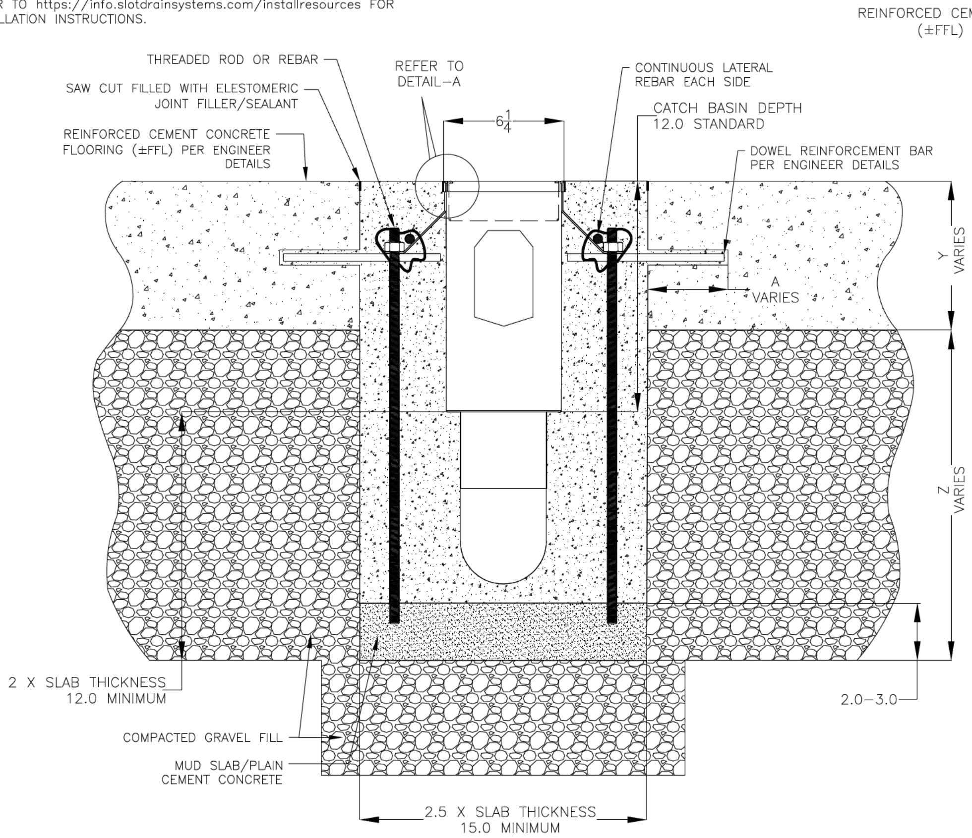
6X6X12 CATCH BASIN INSTALLATION DETAILS
