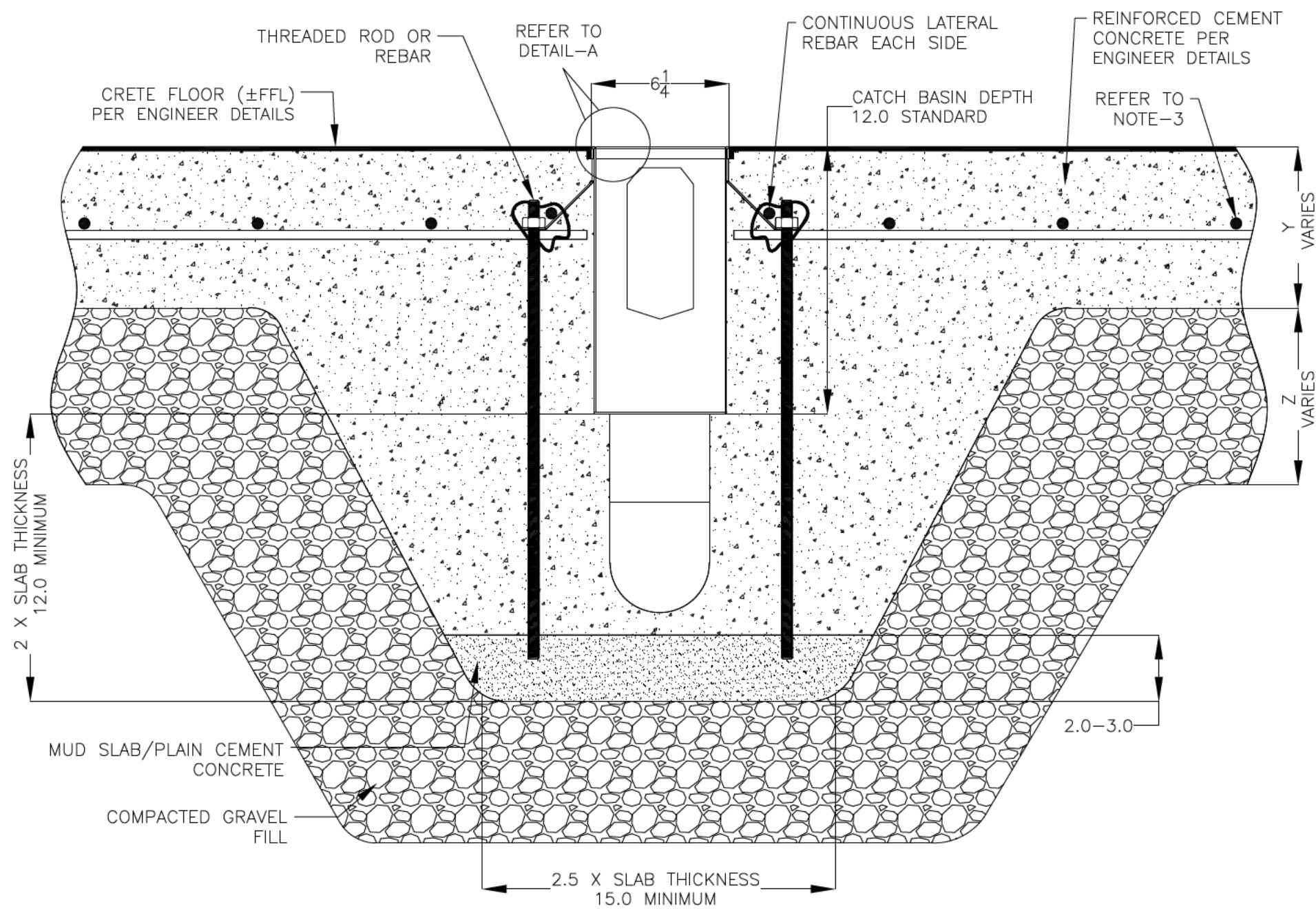
6X6X12 NON FG CATCH BASIN INSTALLATION DETAILS
