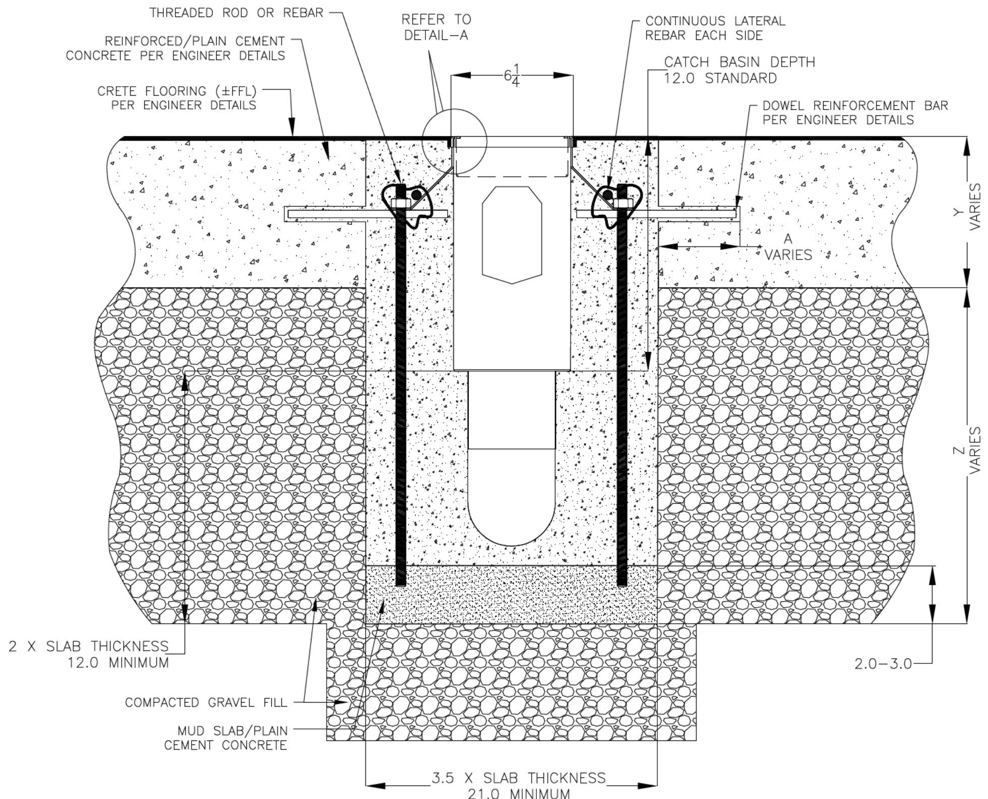
6X12X12 CATCH BASIN INSTALLATION DETAILS
