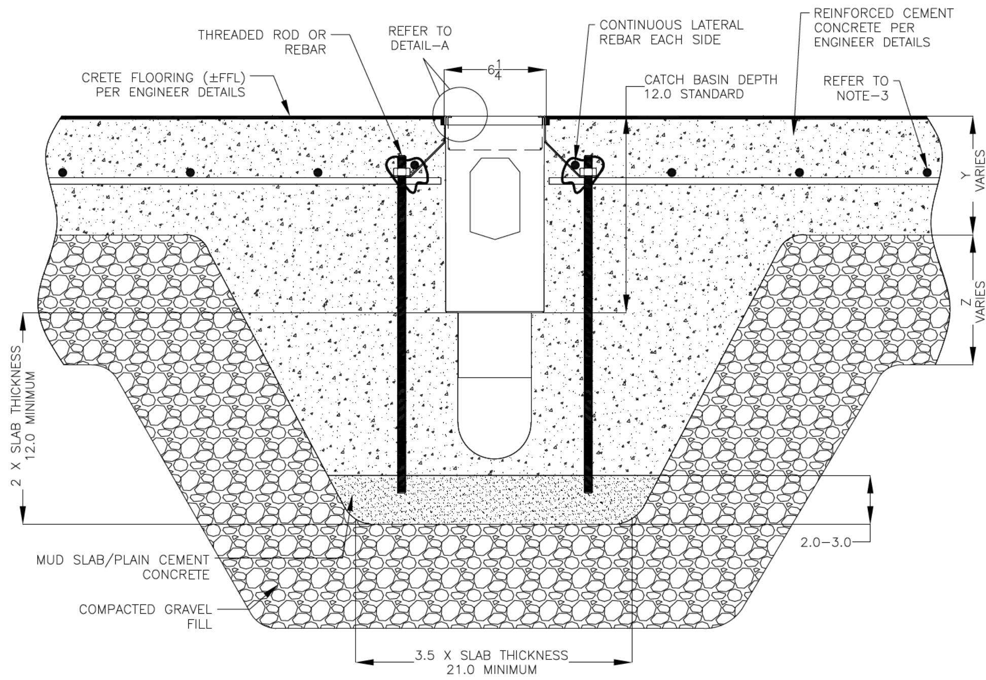
6X12X12 NON FG CATCH BASIN INSTALLATION DETAILS
