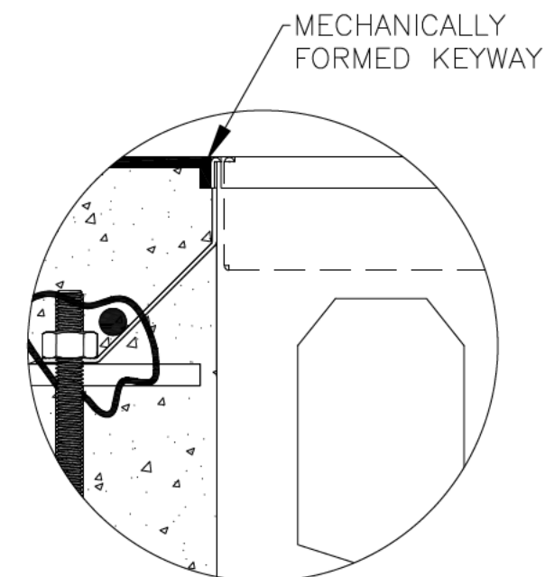
DETAIL-A
