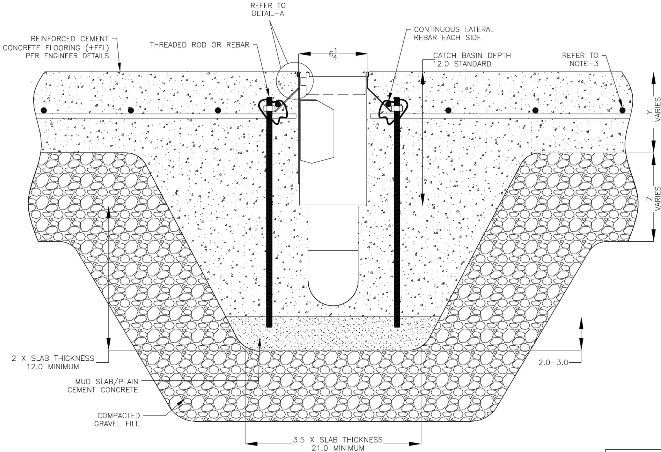
6X6X12 NON FG 4000 CATCH BASIN INSTALLATION DETAILS
