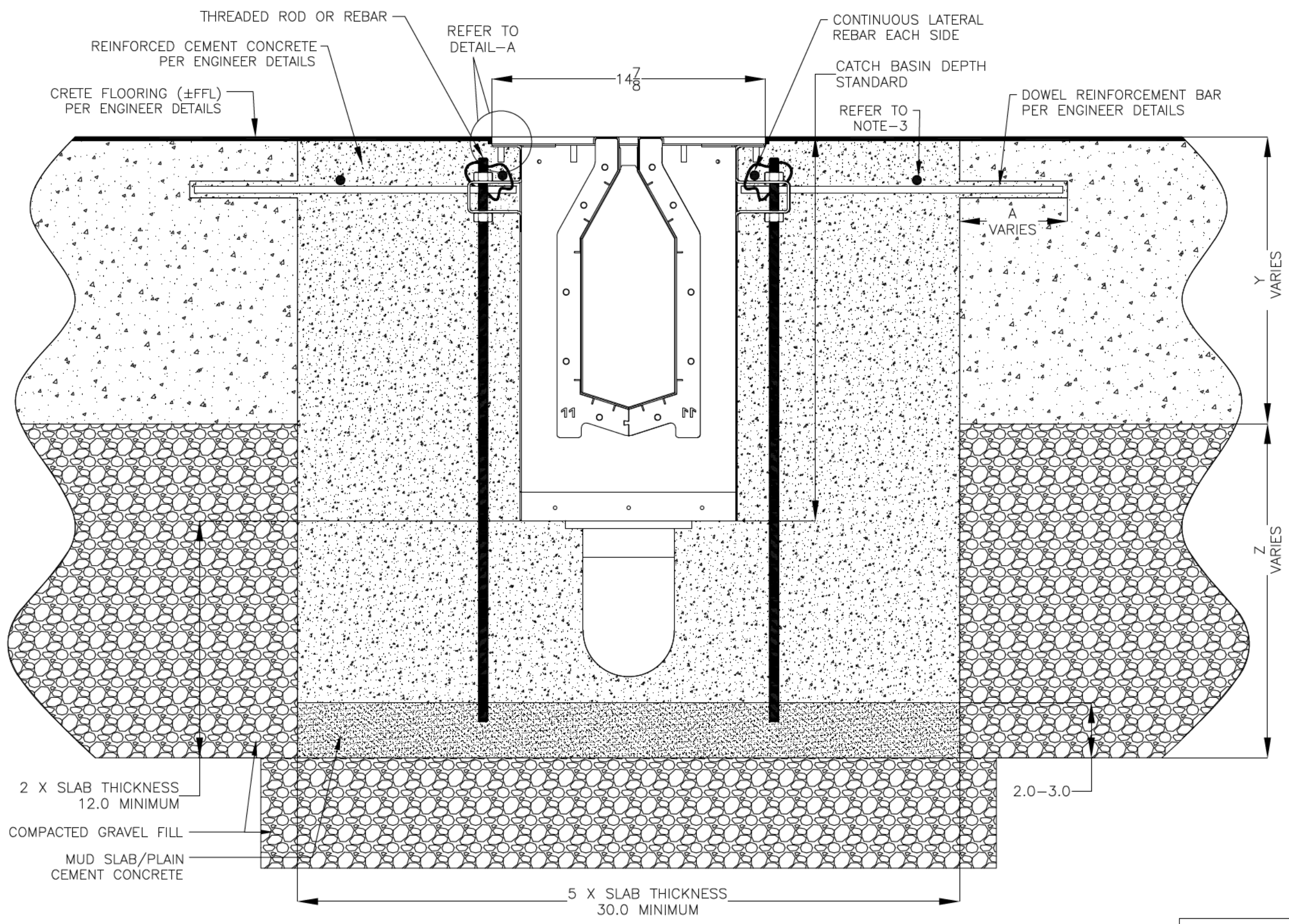
12X12X20 CATCH BASIN INSTALLATION DETAILS
