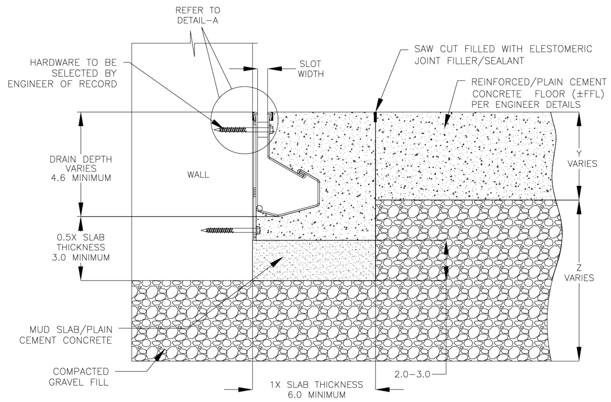
4000 SERIES SLOT DRAIN WALL INSTALLATION DETAILS
