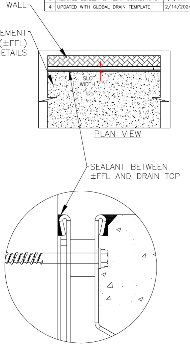
DETAIL-A
