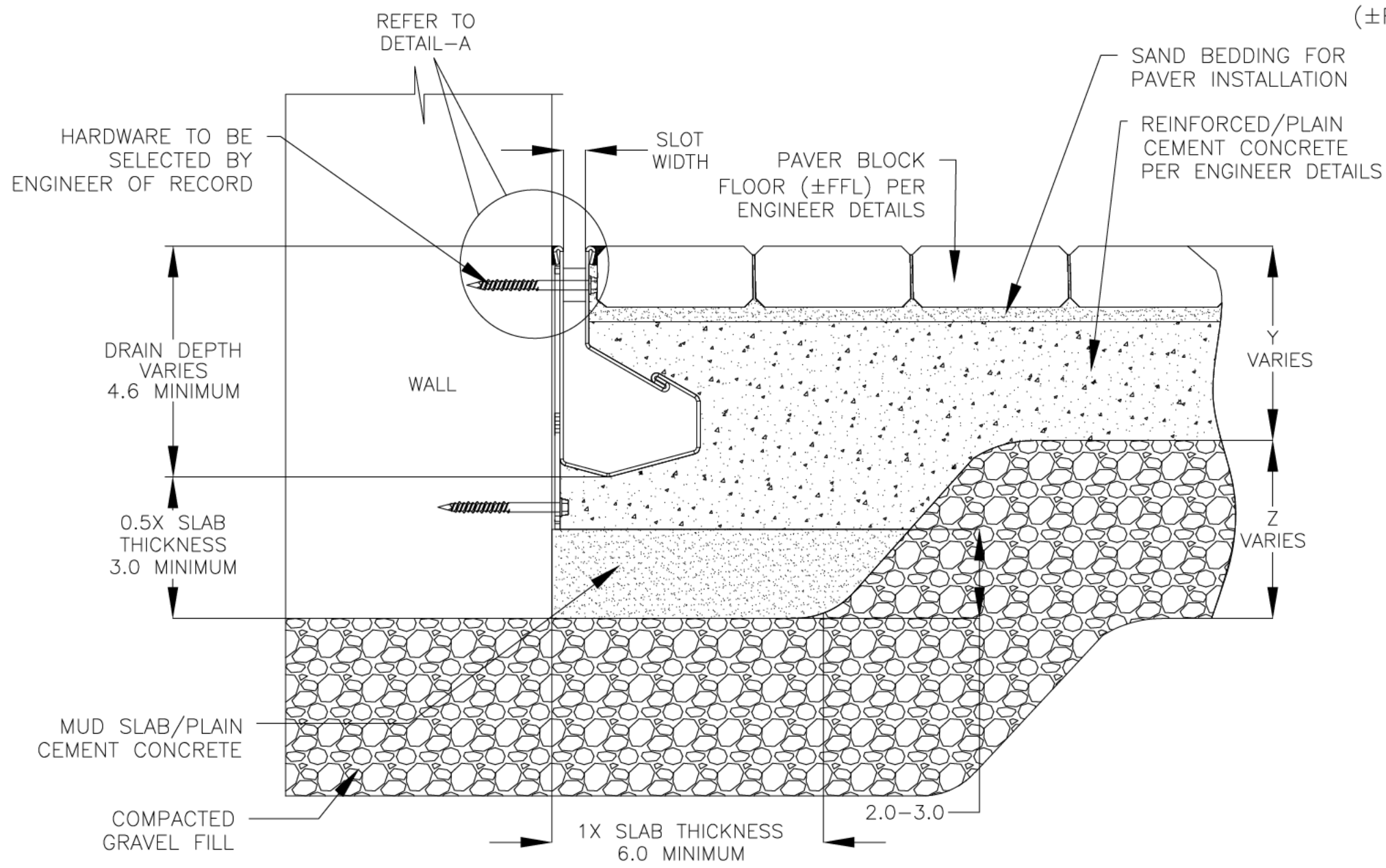
4000 SERIES SLOT DRAIN WALL INSTALLATION DETAILS
