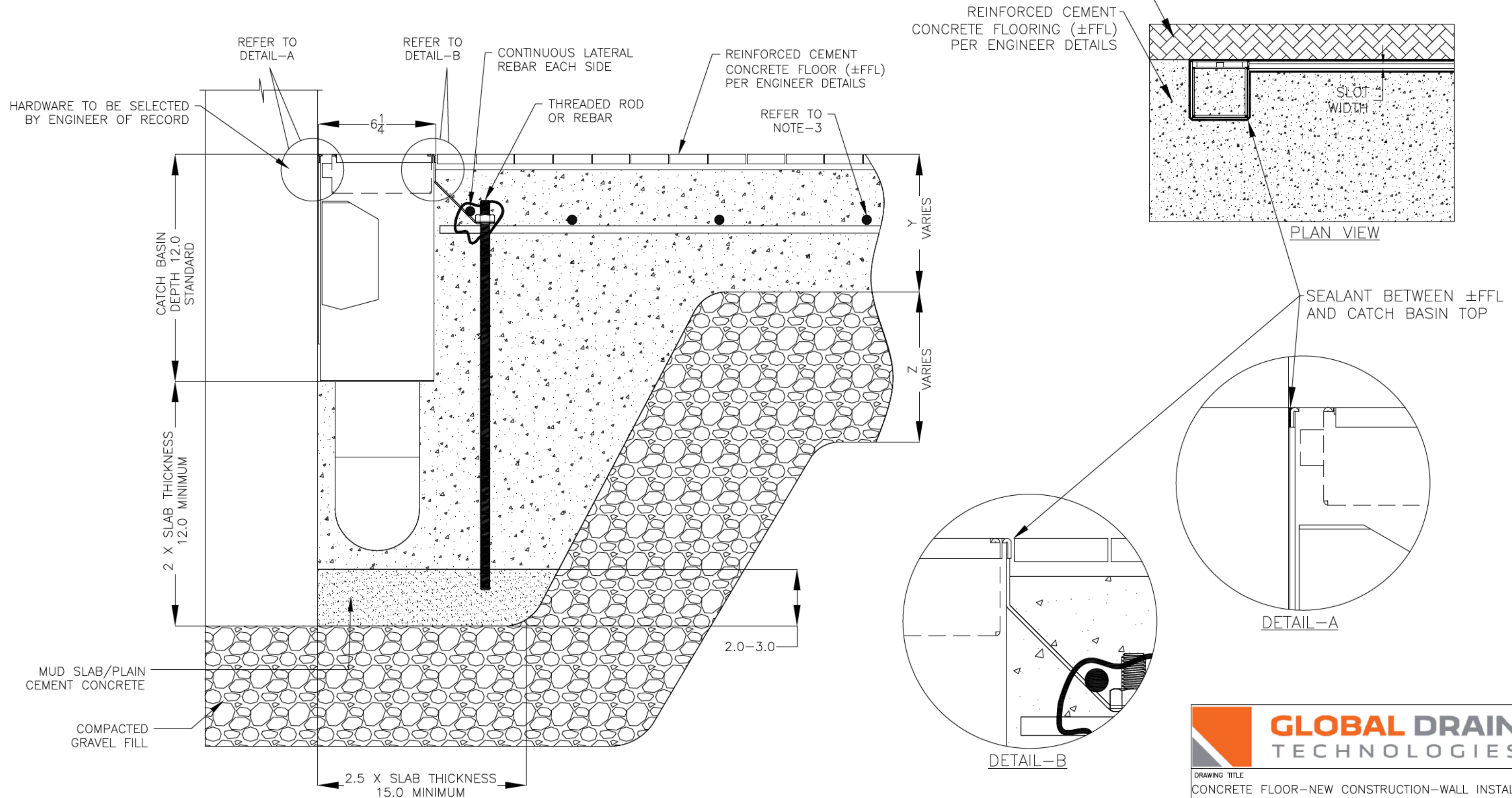
6X6X12 NON FG 4000 CATCH BASIN INSTALLATION DETAILS
